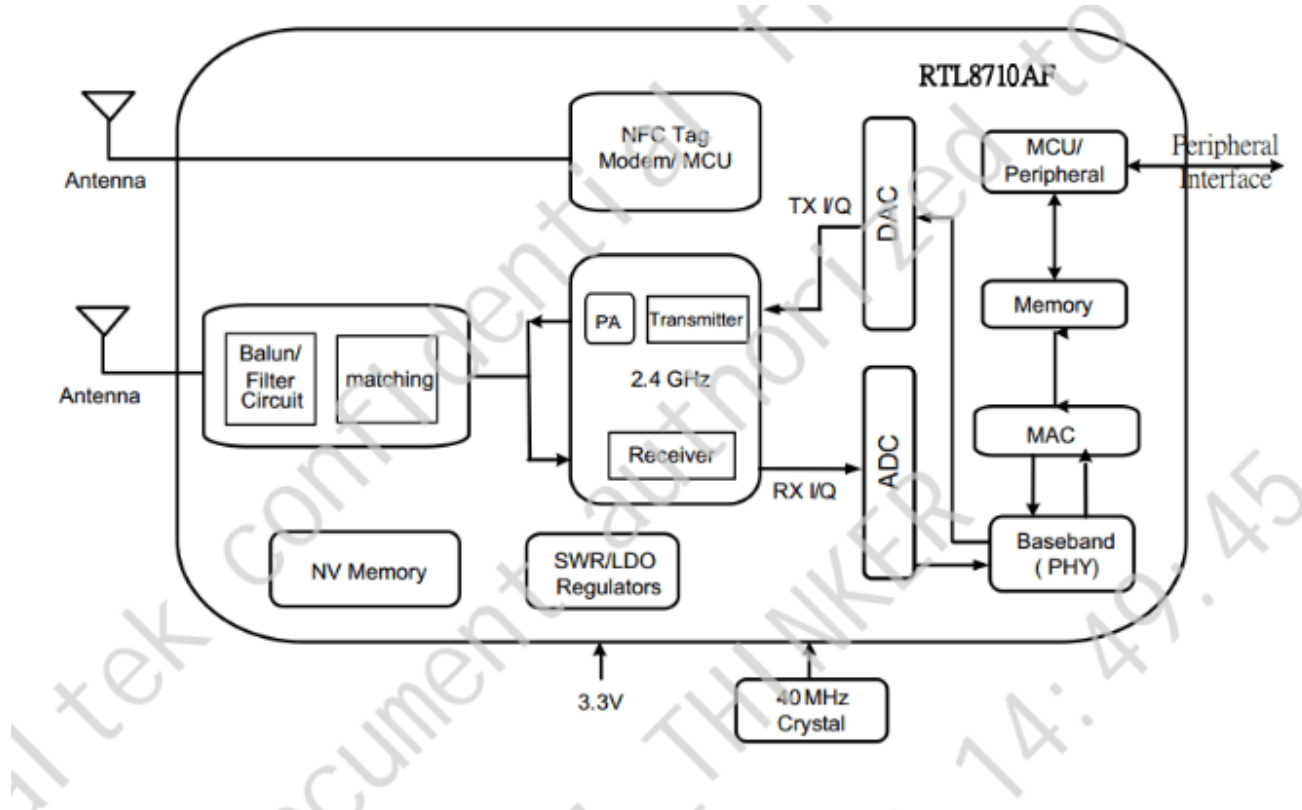
Figure 2. Single-Band 11n (1x1) and NFC Tag Solution
